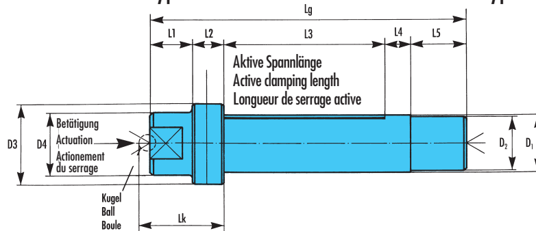
Dimensions and ordering data
