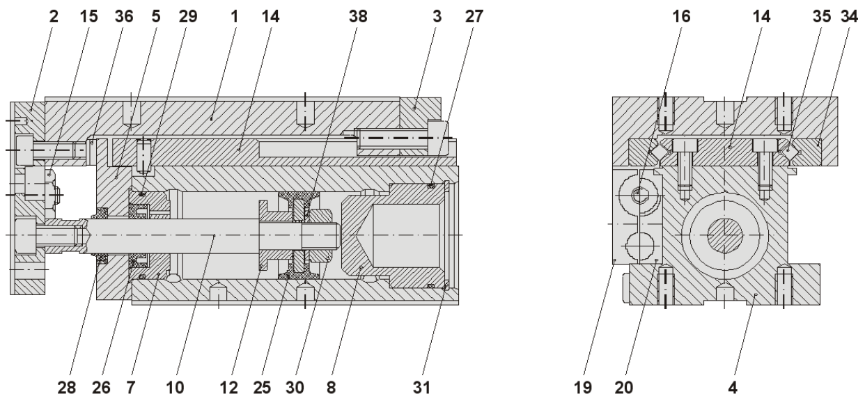
Figure 3: section drawing CLM 50, 100, 200
