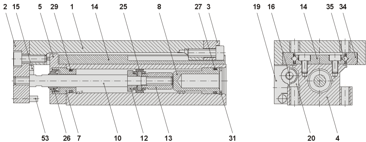
Figure 2: section drawing CLM 25
